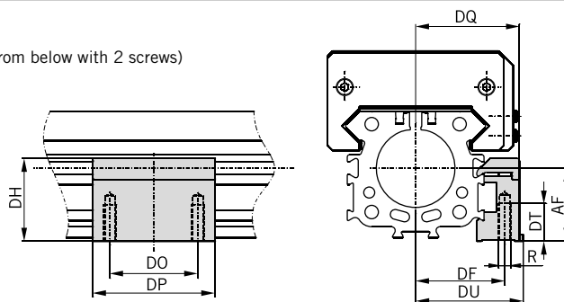
Series OSPP-BG25 to BG50: Type D1BG
