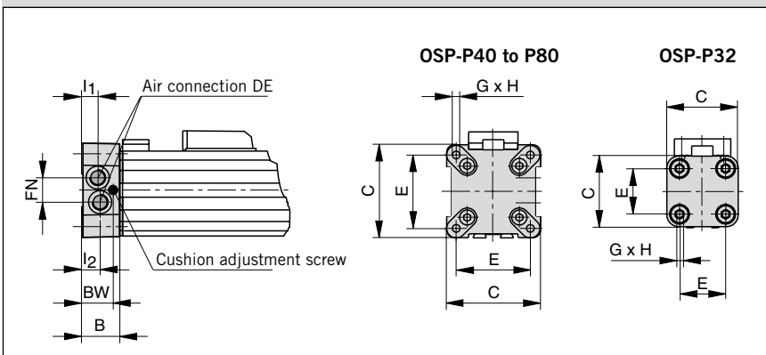
Dimension Table [mm]
