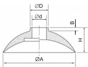
PVG 45 ÷ 85
