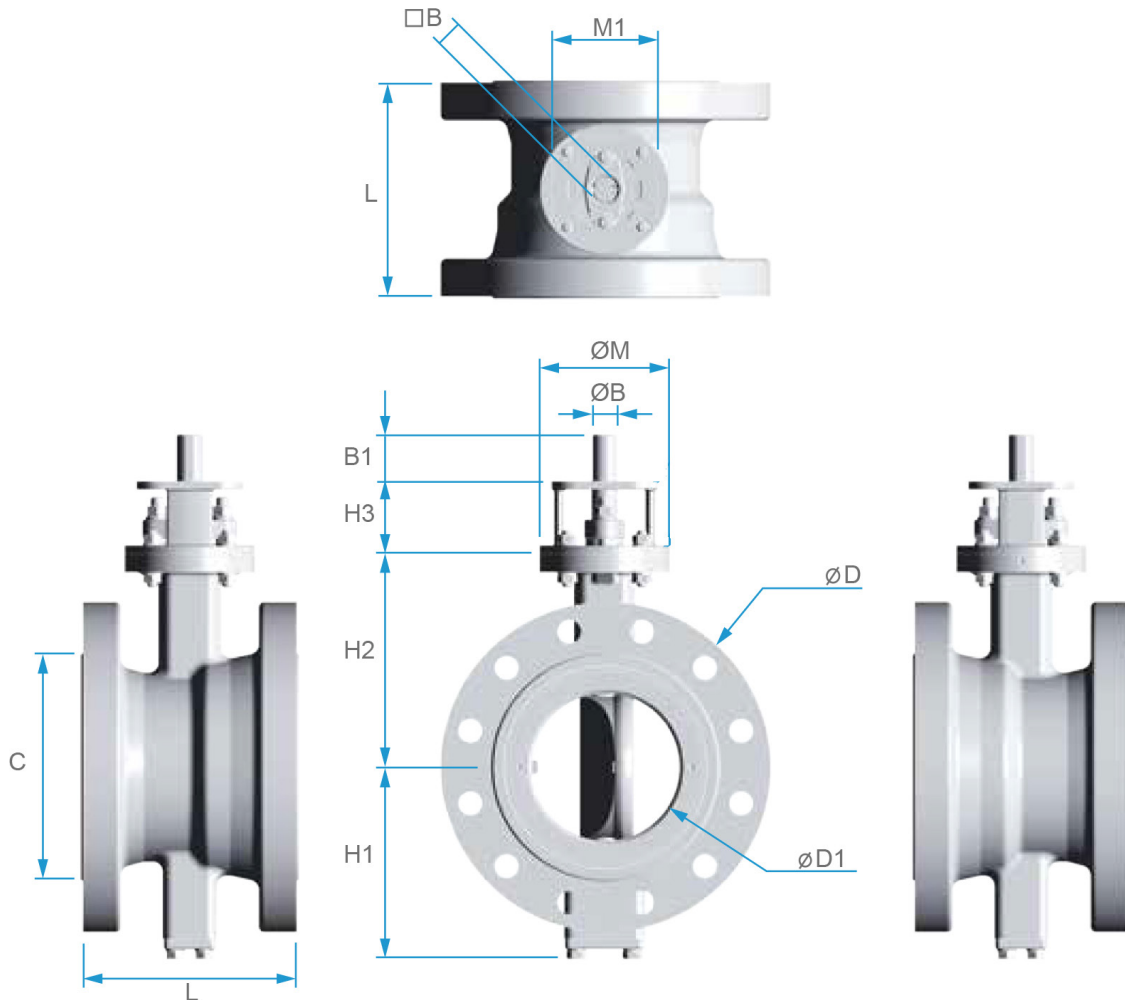
DIMENSIONS (mm)
