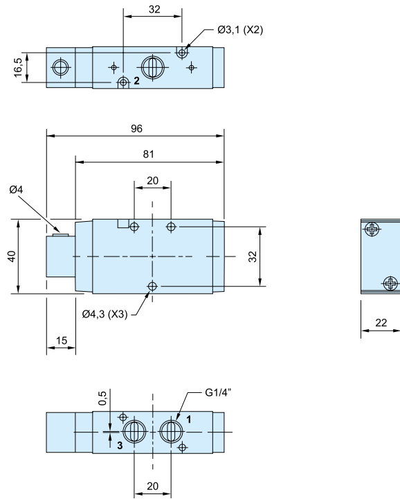
P2LBZ 3/2 Air / Spring
