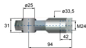
4-M24 Gelenkkopf Spherical end bearing Joint articulé • Forcella snodata Charnela macho articulada
