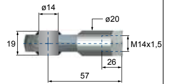
4-M14 Gelenkkopf Spherical end bearing Joint articulé • Forcella snodata Charnela macho articulada
