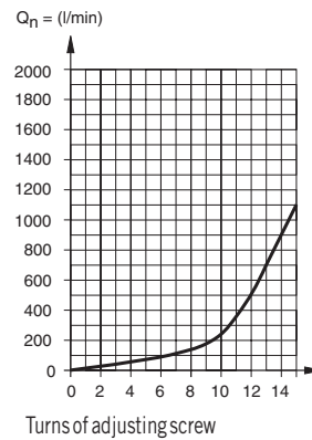
Flow characteristics Type: DRV-3/8
